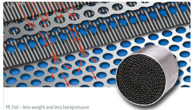
PE Foil – less weight and less backpressure
